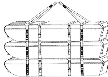
AIRSAFE ADS KOLLI-95, P/N: 2-0430 LOW PROFILE MODULE
